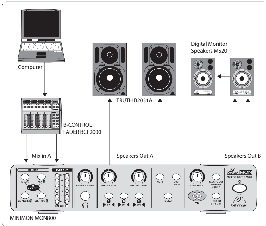
Fig. 2.1: MON800 quick-start set-up
