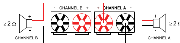
Illustration 2.14: Speaker connection in NORMAL operation mode, using Terminals
