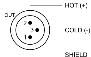
Illustration 4.6: Pin assignment of AES/EBU-OUT
