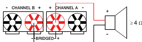
Illustration 2.17: Speaker connection in BRIDGED operation mode, using Terminals
