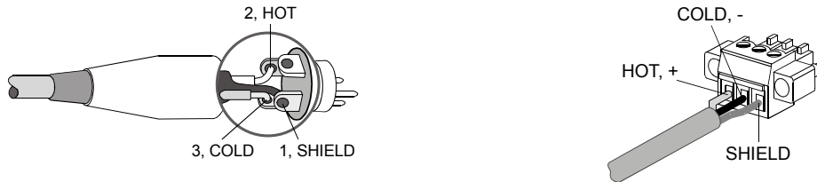
Illustration 2.10: Balanced connection of input
