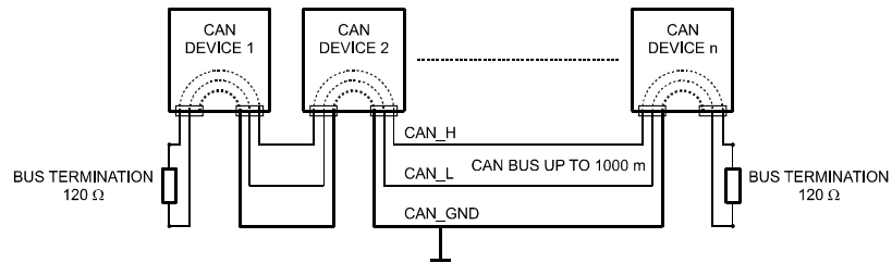
Illustration 4.10: Bus Topology of the CAN bus
