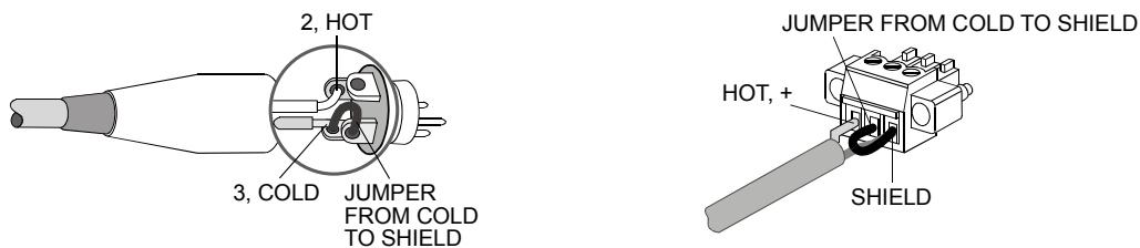
Illustration 2.11: Unbalanced connection of input
