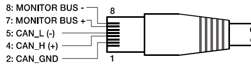
Illustration 4.8: Pin-assignment of CAN plug
