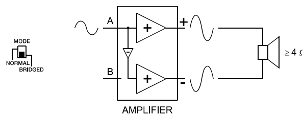
Illustration 2.9 : Mode BRIDGED
