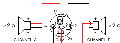
Illustration 2.15: Bi-Amp speaker connection in NORMAL operation mode, using only the Speakon A connector
