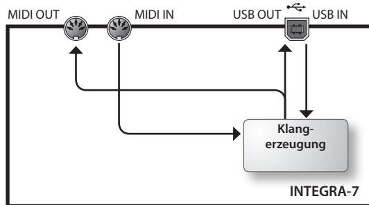
USB-MIDI Thru=OFF
