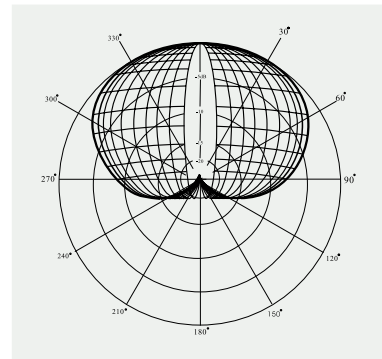
CARDIOID POLAR PATTERN
