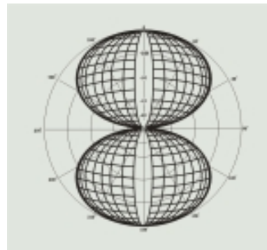
FIGURE-8 POLAR PATTERN
